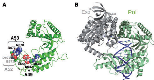
Fig. 2. A model of HHV-1 UL8c compared with E.coli PolIII. (A) UL8c and its mutants that affect binding to UL52. Mutated residues are shown in space-filling representation (carbon atoms, gray/white; nitrogen, blue; oxygen, red) and are labeled. (B) Crystal structure of E.coli PolIII complexed with DNA. Polymerase (Pol) and exonuclease (Exo) domains are colored in green and gray, respectively
